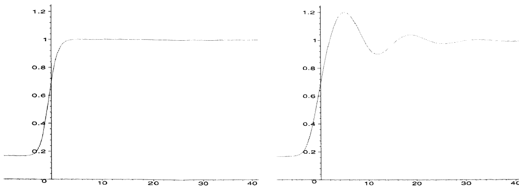
(a) Monotone profile: \varepsilon = \varepsilon^* - 0.01 \approx 0.048 .
